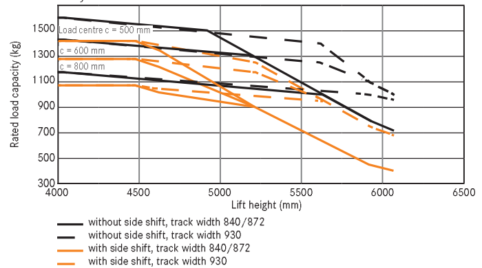
Basic capacities RX 50-16 triplex mast, SE tyres
